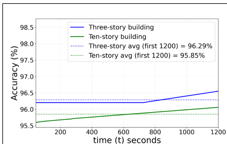
Figure 4. SPARK Prediction Accuracy over time.
