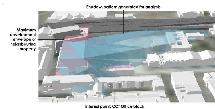
Figure 91: Shadow analysis to inform the positioning of solar panels on CCT building for Facilities Management
