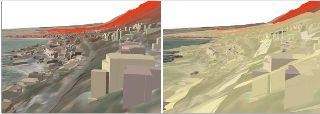
Figure 6: Ground Level Map 2019 5m DEM and 2m contours visualised in 3D (left) and then offset to show a parallel surface of the Single Residential height limit of 10m above EGL (GLM 2019) (right).
